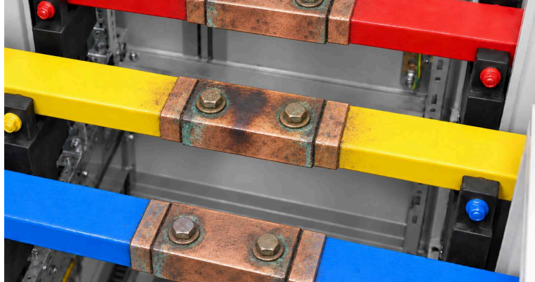
BEFORE: SPLICE-ൽ CORROSION
