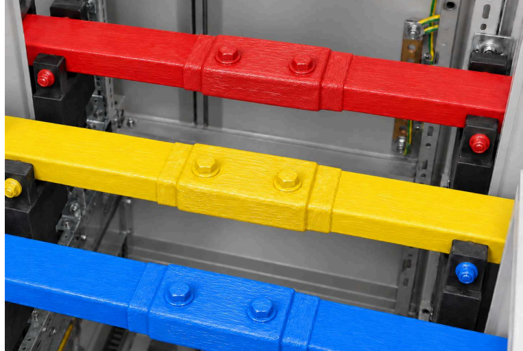
بعد میں: JOINT &amp; BOLTS COATED
